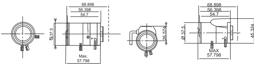
Tokina Manuel İris Megapiksel Lens
